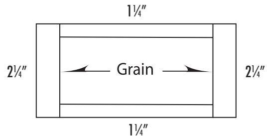
TYPICAL 5-PIECE COPE & STICK DRAWER FRONT
