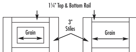
DF-324 (Raised Panel) Minimum Width 8 3/4"
