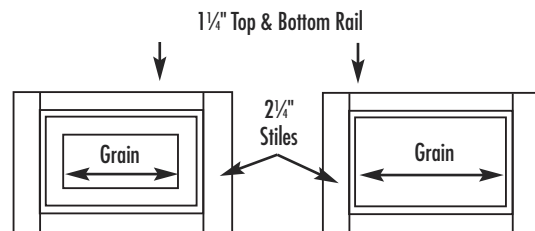
DF-301 (Raised Panel) Minimum Width 7 1/4"
