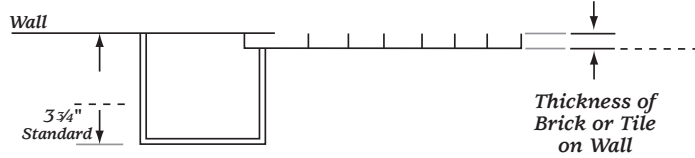
Top View of Leg
