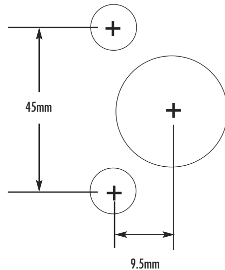
Hinge Bore Pattern #HBP 100
