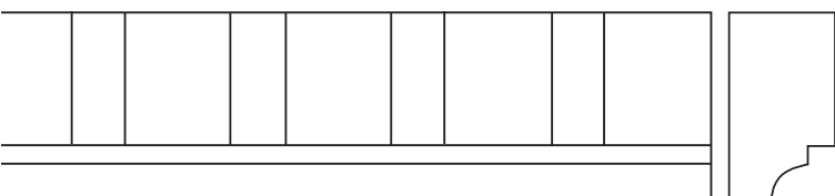
V-104 7/8" Dentil Moulding
